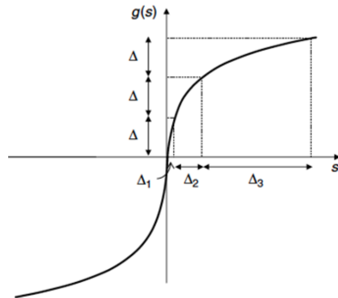
Companding function for non uniform PCM
